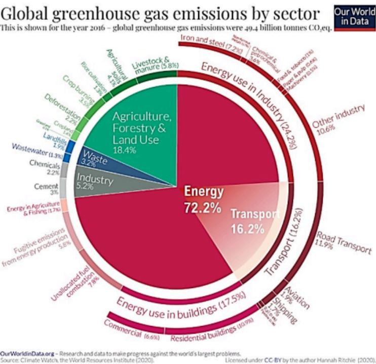
Fig. 2. Global greenhouse gas emissions by sector
