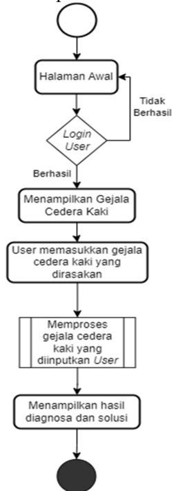
Gambar 2. Flowchart Sistem
