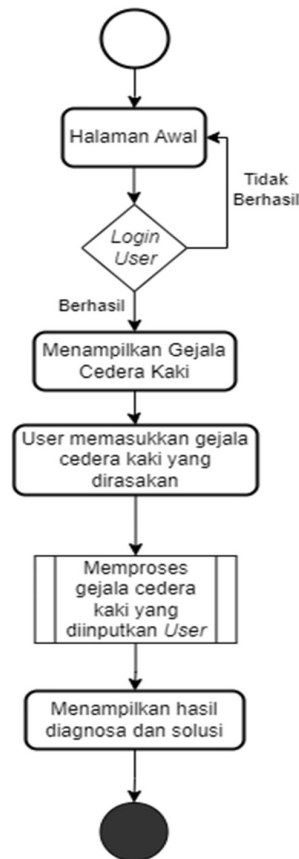
Gambar 2. Flowchart Sistem
